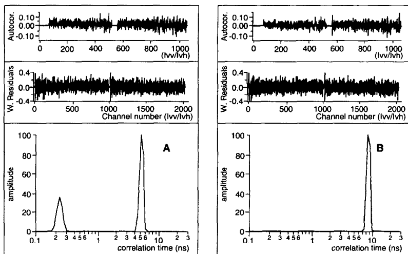
Fig. 5. Amplitude profile of the rotational correlation times of (A) fresh and (B) irradiated solution of cutinase, recovered by MEM analysis of the decay of the fluorescence anisotropy. Values obtained for barycenters (relative areas in %) of the peaks are for the fresh solution: 0.24 ns (33%), 5.5 ns (67%), and for the irradiated solution: 8.9 ns (100%). Chi square amounts to 1.38 (A) and 2.11 (B). The top panels show the weighted residuals and autocorrelation of the residuals.
