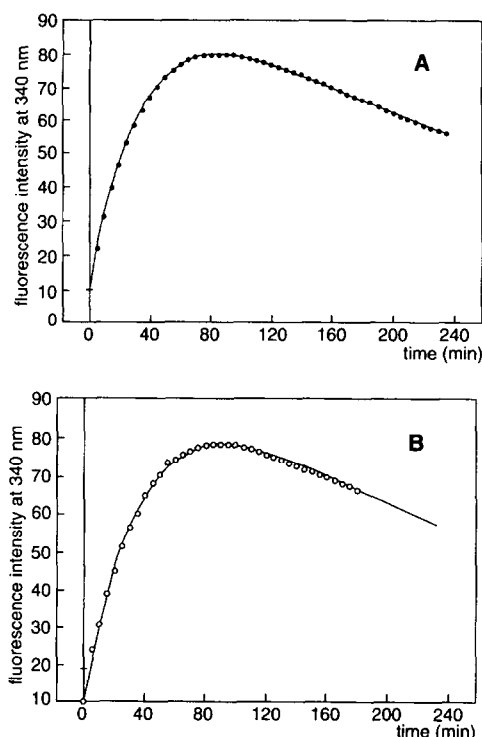
Fig. 2. Intensity of the fluorescence at 340 nm, emitted by a 2.5 \mu\text{M} solution of cutinase solution as a function of time under conditions of constant irradiation in the spectrofluorimeter at (A) 20°C and (B) 40°C. The lines represent the best fit of the biexponential function in Eq. (1) to the experimental points. Fit parameters are: k_r = 0.026 \text{ min}^{-1} , k_d = 0.0038 \text{ min}^{-1} (A) and k_r = 0.023 \text{ min}^{-1} and k_d = 0.0039 \text{ min}^{-1} (B).
