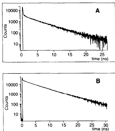
Fig. 3. Decay of the fluorescence intensity after pulse excitation of (A) fresh and (B) irradiated 10 \mu M solution of cutinase.
