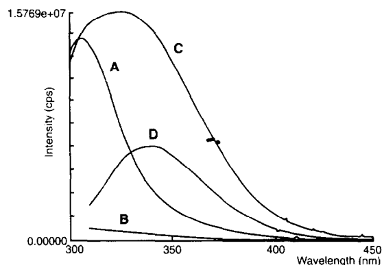
Fig. 1. Fluorescence spectra of 2.5 \mu M solutions of cutinase in 10 mM Tris/NaCl buffer pH 9. Freshly prepared solutions excited with (A) 280 and (B) 295 nm light, irradiated solutions excited with (C) 280 and (D) 295 nm light.
